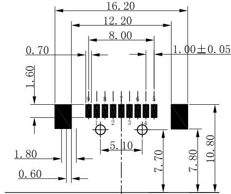
PCB EDGE RECOMMENDED PCB LAYOUT
