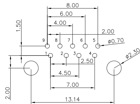
CONNECTOR FRONT EDGE PREFERENCE PCB LAYOUT
