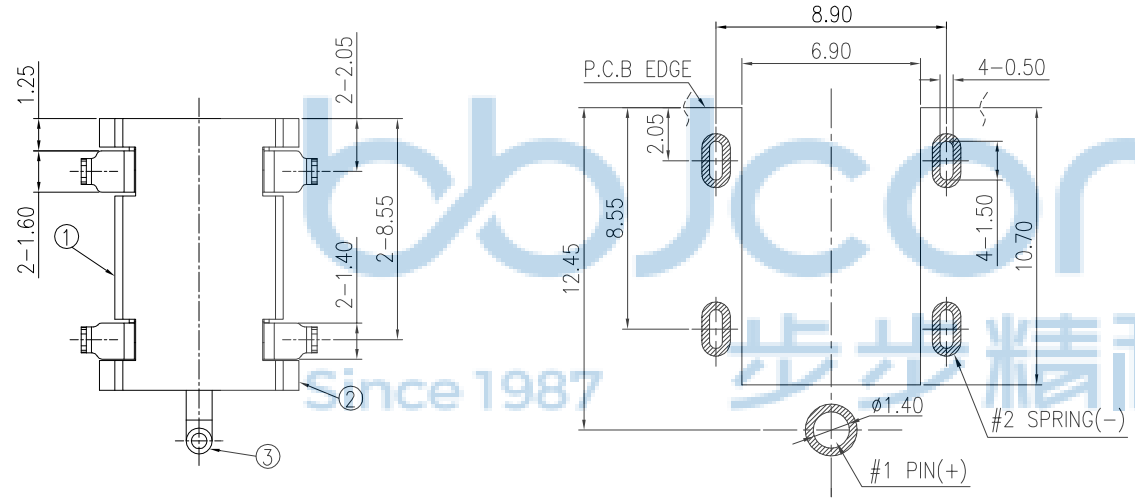
RECOMMENDED PCB LAYOUT TOP VIEW (TOLERANCE:±0.05)
