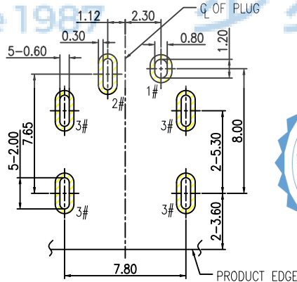
RECOMMENDED PCB LAYOUT TOP VIEW TOLERANCE: \pm 0.05
