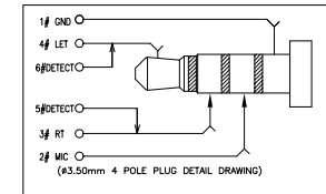
( \phi 3.50 mm 4 POLE PLUG DETAIL DRAWING)
