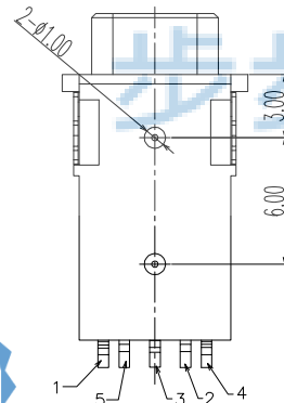
SCHEMATIC (PLUG OUT)
