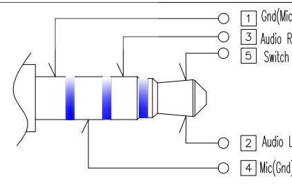
SCHEMATIC (PLUG IN)
