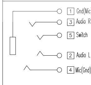
SCHEMATIC (PLUG OUT)
