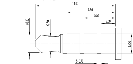
(φ3.50mm 4 POLE PLUG DETAIL DRAWING)
