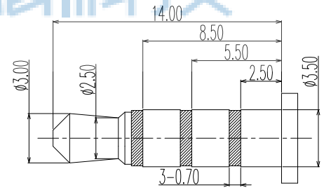
(φ3.50mm 4 POLE PLUG DETAIL DRAWING)
