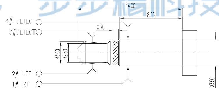
( \phi 3.50 mm 4 POLE PLUG DETAIL DRAWING)
