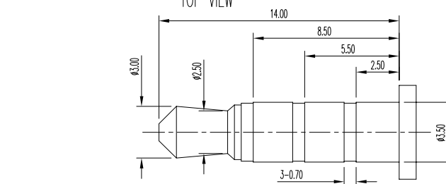
(φ3.50mm 4 POLE PLUG DETAIL DRAWING)
