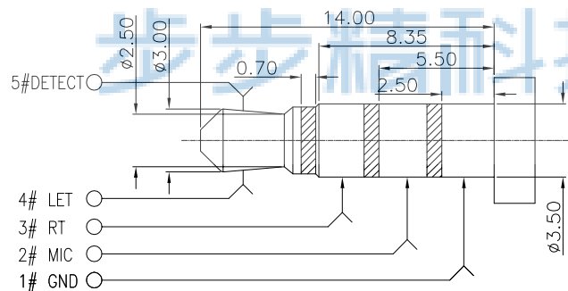
(Ø3.50mm 4 POLE PLUG DETAIL DRAWING)
