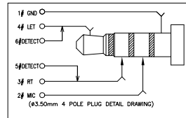
(ø3.50mm 4 POLE PLUG DETAIL DRAWING)
