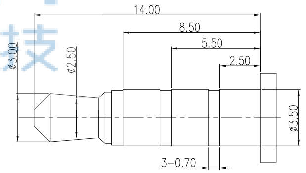
(φ3.50mm 4 POLE PLUG DETAIL DRAWING)
