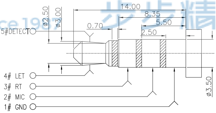
(φ3.50mm 4 POLE PLUG DETAIL DRAWING)
