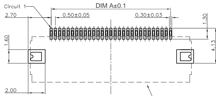
RECOMMENDED P.C.B PATTERN LAYOUT
