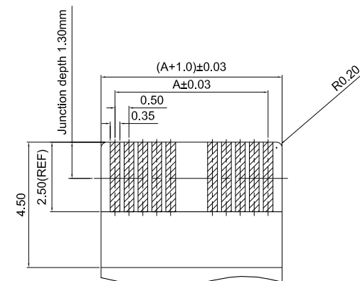
APPLICABLE FPC/FFC T=0.30 ±0.03
