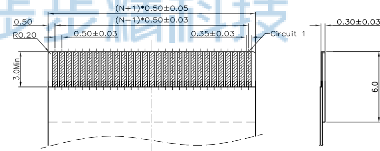
RECOMMENDED FPC/FPC DIMENSION
