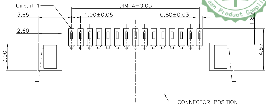
RECOMMENDED P.C.B. PATTERN LAYOUT
