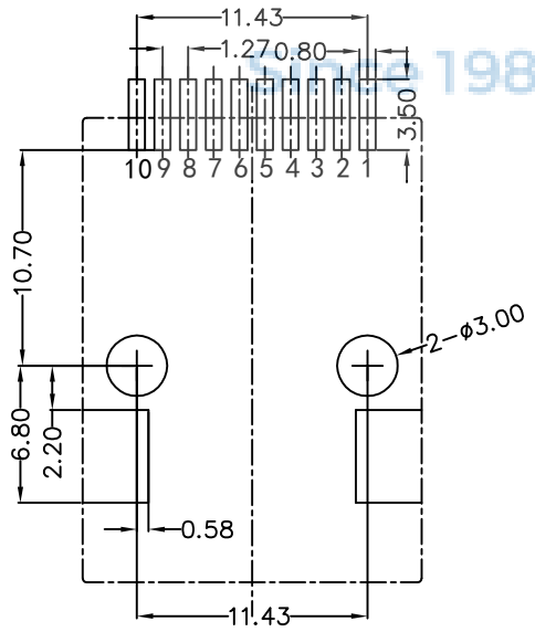
RECOMMENDED PCB LAYOUT VIEWED FROM COMPONENT SIDE
