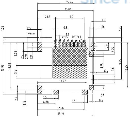
RECOMMENDED PCB PATTERN LAYOUT(TOP VIEW) TOLERANCE: ±0.05
