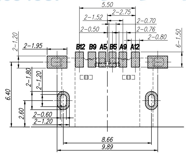
P.C.B LAYOUT VIEW TOLERANCE ±0.05
