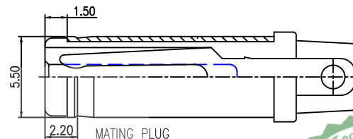
MATING PLUG
