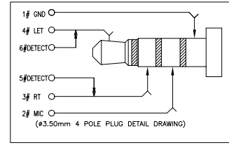
(ø3.50mm 4 POLE PLUG DETAIL DRAWING)
