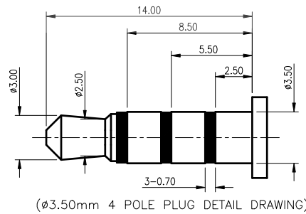
(φ3.50mm 4 POLE PLUG DETAIL DRAWING)
