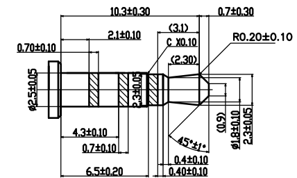
(Ø2.50mm 4 POLE PLUG DETAIL DRAWING)
