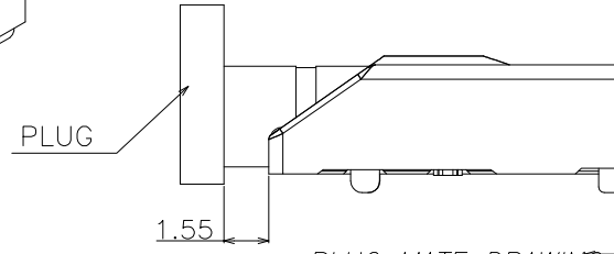
PLUG MATE DRAWING
