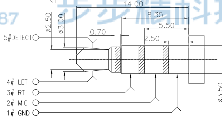
( \phi 3.50 mm 4 POLE PLUG DETAIL DRAWING)
