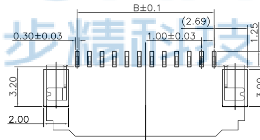
RECOMMENDED METAL MASK PATTERN (THICKNESS 0.10MM)
