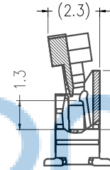
SECTION A-A Without cover
