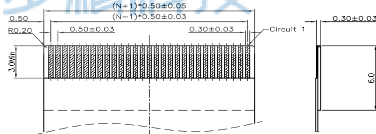
RECOMMENDED FPC/FFC DIMENSION
