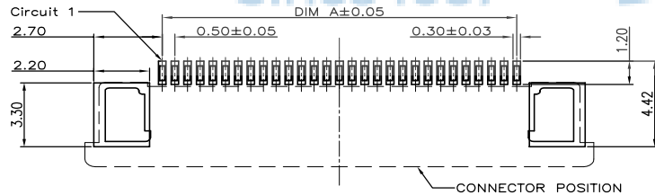
RECOMMENDED P.C.B. PATTERN LAYOUT
