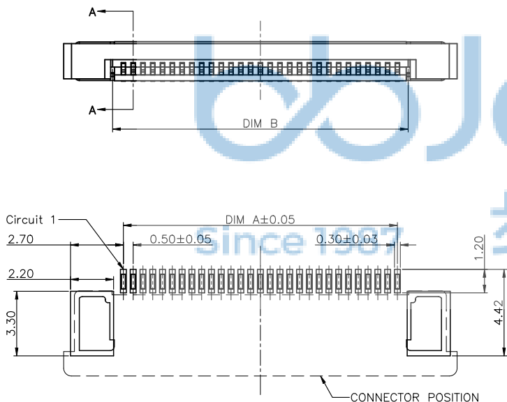
RECOMMENDED P.C.B PATTERN LAYOUT
