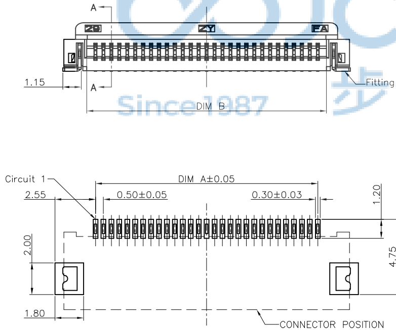
RECOMMENDED P.C.B PATTERN LAYOUT
