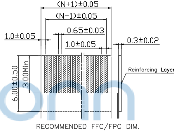
RECOMMENDED FFC/FPC DIM.
