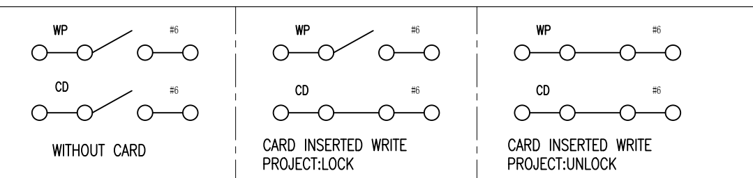
Circuit Diagram for Detect SW
