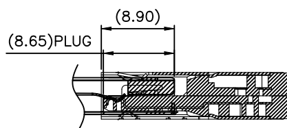
MATING DRAWING
