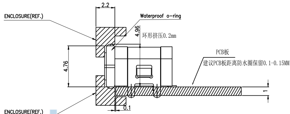
RECOMMENDED SCHEMATIC DRAWING OF CONNECTOR MATCH CHASSIS
