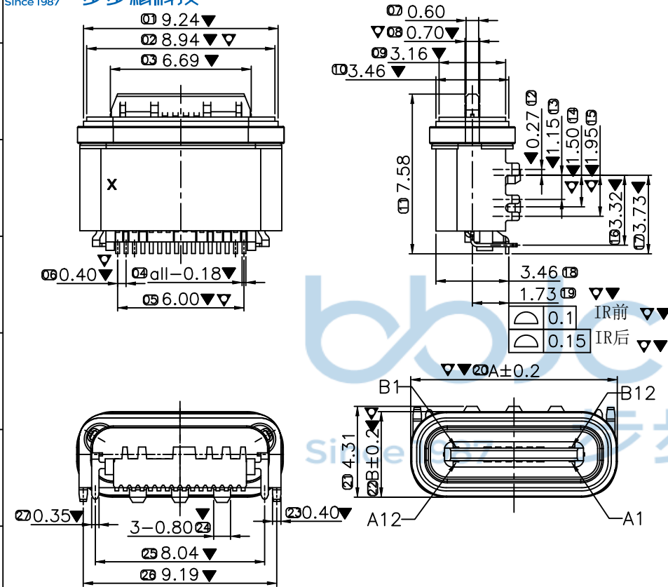
TYPE-C 16P 5.4L
