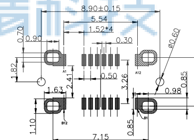
RECOMMENDED P.C.B. LAYOUT (T:1.00mm) TOLERANCE UNSPECIFIED ±0.05mm
