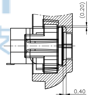
Interferebce_Fit Size
