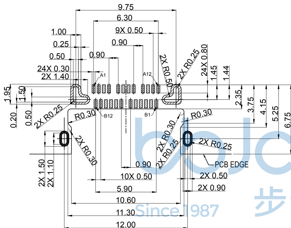
RECOMMENDED PCB LAYOUT (Tolerance= \pm 0.05 )
