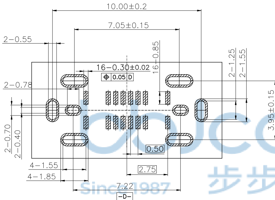
RECOMMENDED PCB LAYOUT (SCALE 2:1) TOLERANCE UNSPECIFIED \pm 0.05\text{mm}
