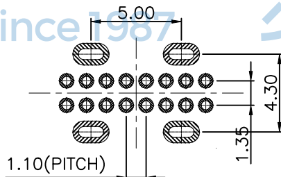
RECOMMENDED PCB LAYOUT(TOP VIEW) (GENERAL TOLERANCE±0.05)
