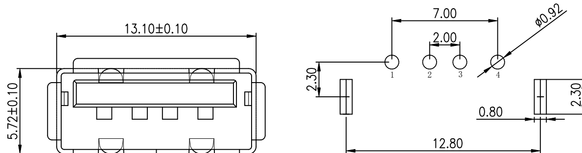
P. C. B LAYOUT
