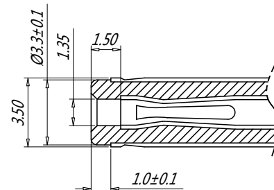
MATE PLUG
