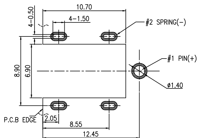
RECOMMENDED PCB LAYOUT TOP VIEW (TOLERANCE:±0.05)
