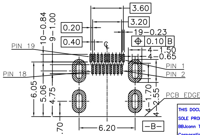
RECOMMENDED PCB LAYOUT(.XX±0.05) CONNECTOR SIDE(TOP VIEW)
