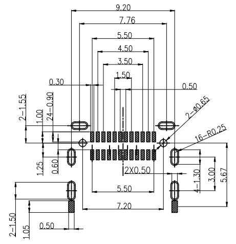
RECOMMENDED P.C.B LAYOUT (COMPONENT SIDE) PCB THICKNESS: 2.0±0.05mm
