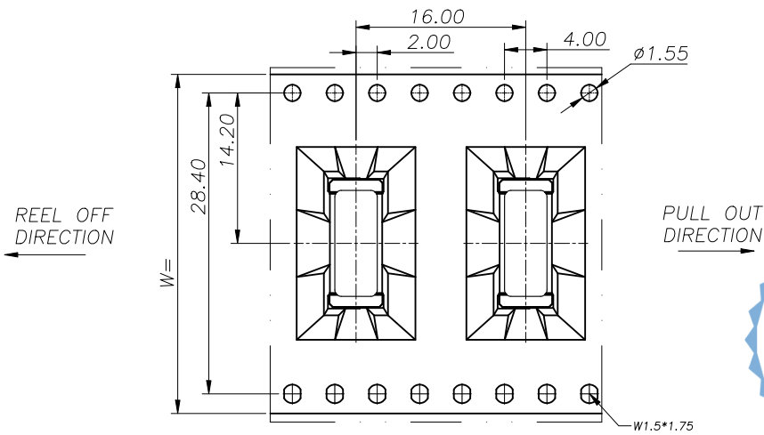
DETAIL X
