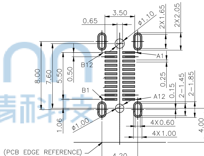
RECOMMENDED P.C.B LAYOUT TOLERANCE ± 0.05mm (TOP VIEW)
