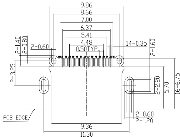
P.C.B LAYOUT VIEW TOLERANCE ±0.05
