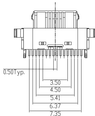
USB TYPE-C PIN ASSIGNMENTS
