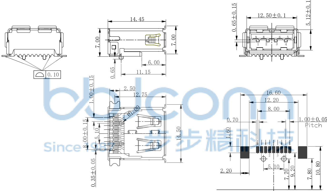
PCB EDGE RECOMMENDED PCB LAYOUT
